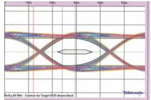
Approved Eye-Pattern diagram, 5m JenTech HDMI Cable
